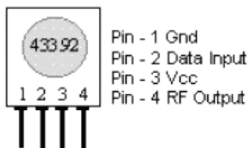
Figure 3. RF-434 Pin Diagram
